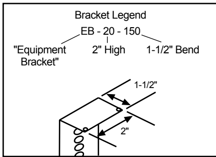
Measuring for Equipment Brackets
